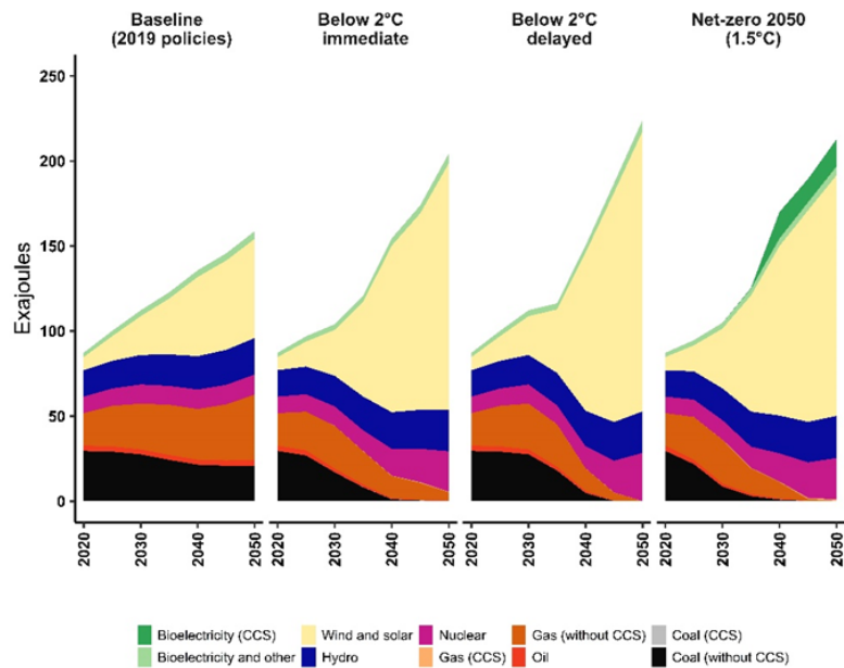
Figure 7: Global electricity generation in different scenarios
