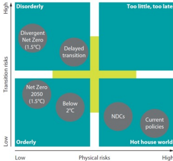
Figure 4: NGFS scenarios Framework
