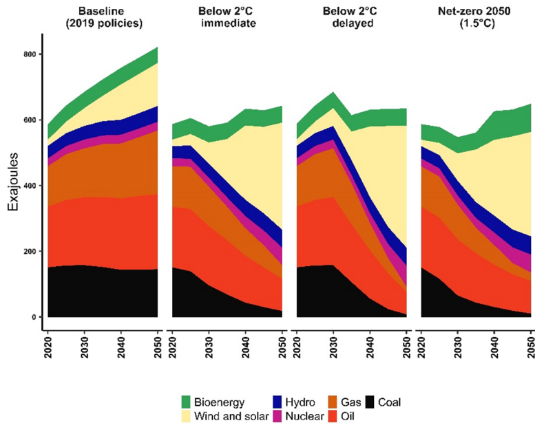
Figure 6: Global primary energy in different scenarios
