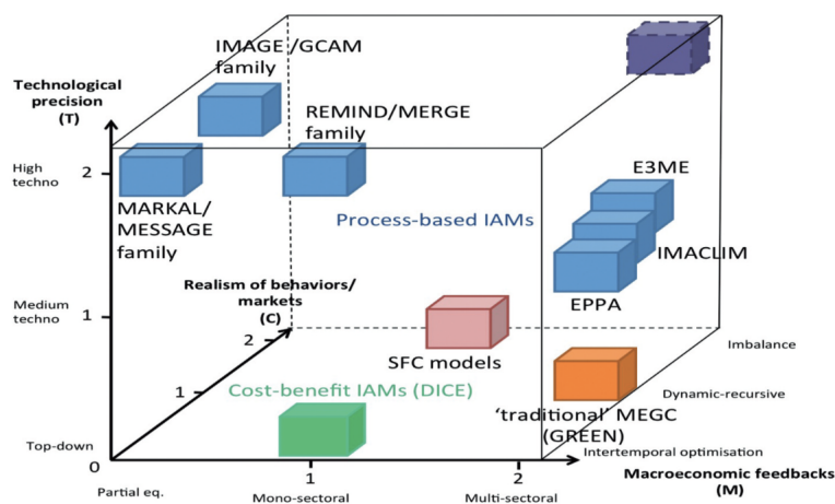
Figure 2: Taxonomy of energy/climate models in terms of three axes of characteristics
