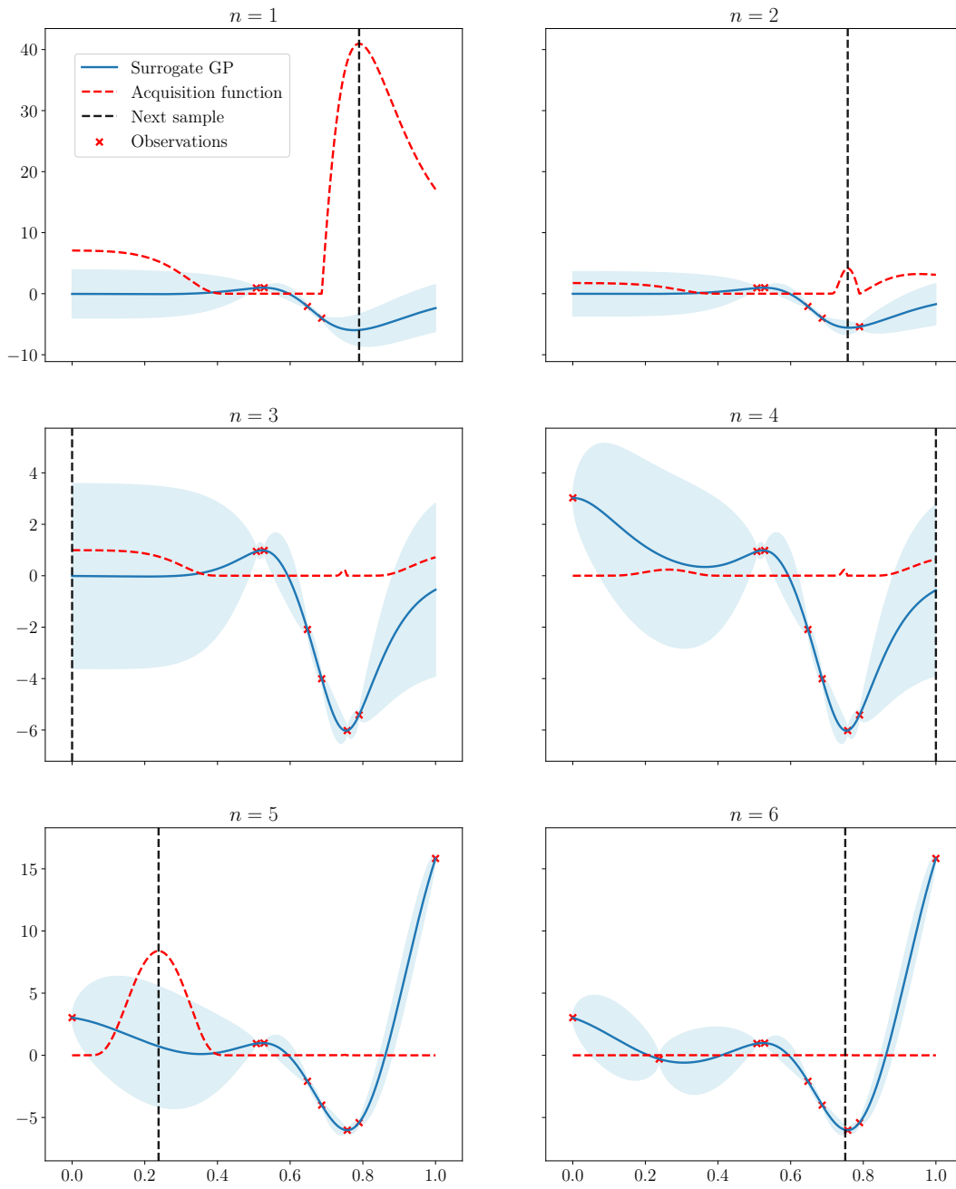
Figure 7: Iterations of the Bayesian optimization
